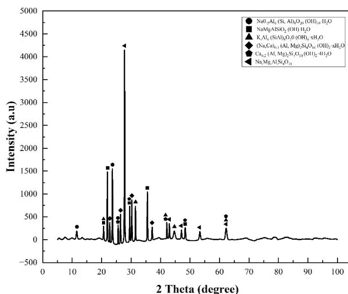
Figure 2. Monmorillonite diffraction pattern using XRD from Marapi volcanic ash
