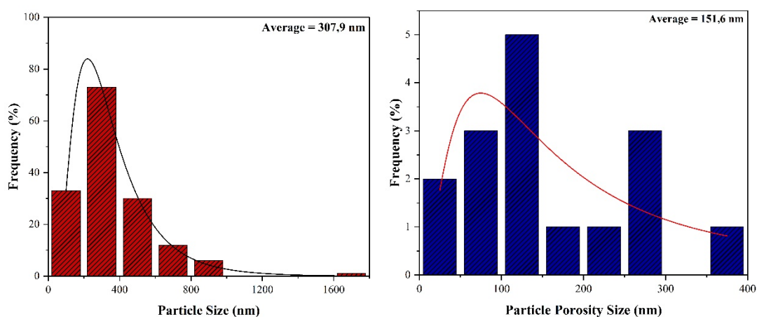
Figure 5. Results of SEM Analysis of Marapi volcanic ash (a) Particle size analysis (b) Particle porosity size analysis
