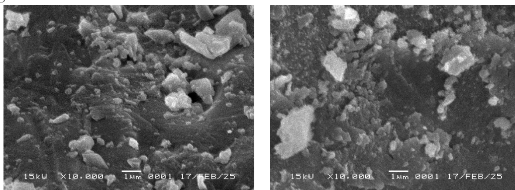
Figure 4. SEM image of Marapi volcanic ash morphology
