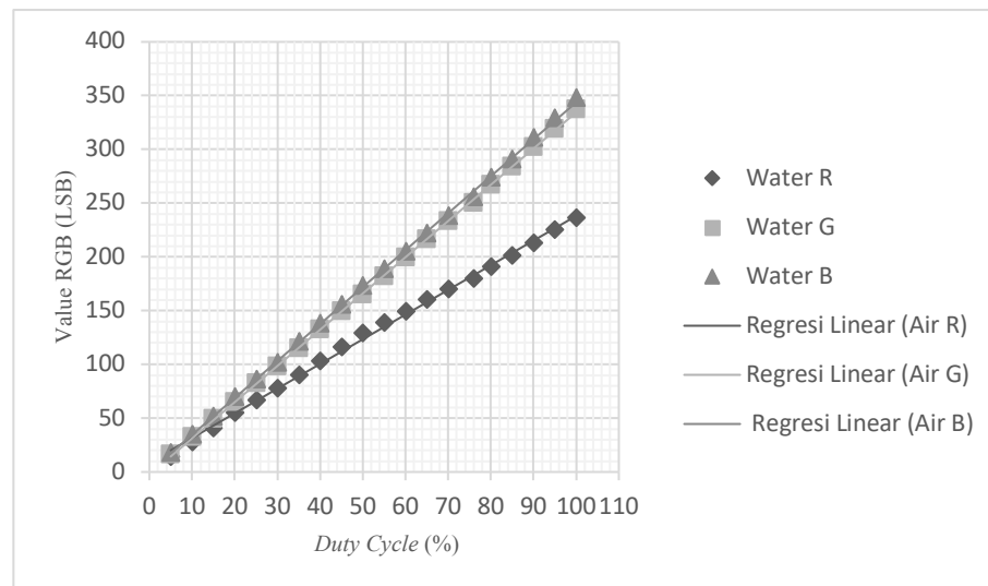
Figure 4. TCS34725 sensor as a function of duty cycle on the distilled water tube
