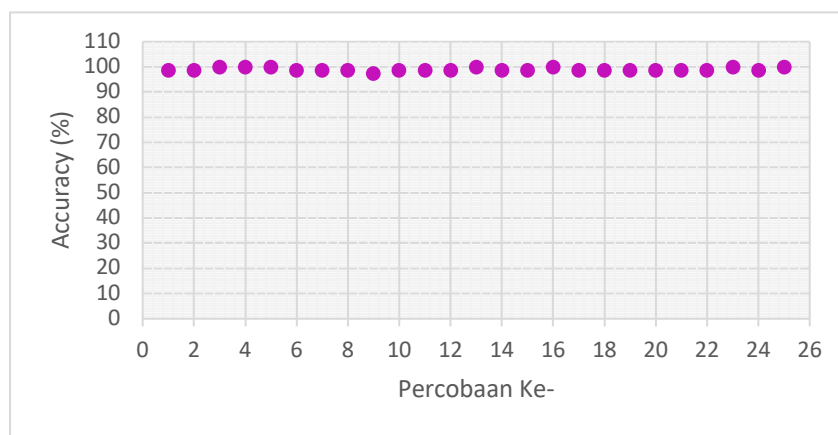
Figure 8. Accuracy of water pH measurement tools for aquaculture
