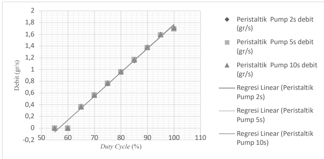
Figure 5. Relationship between duty cycle and water discharge in sample peristaltic pump
