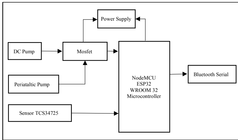
Figure 1. Block diagram of water pH measuring instrument
