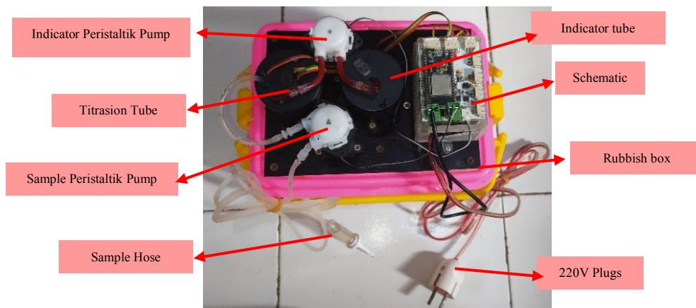
Figure 2. Design of a water pH measuring device
